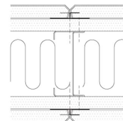
Gypsum Board Joint of Type 1290
