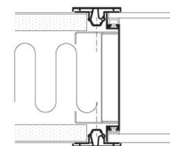
Gypsum Board/Glass Joint
