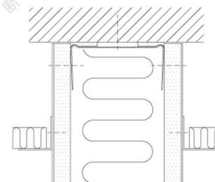
Fixed Ceiling Connection
