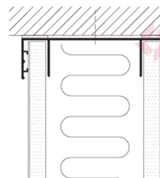
Conventional Fixed Connection
