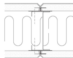
Gypsum Board Joint of Type 1090
